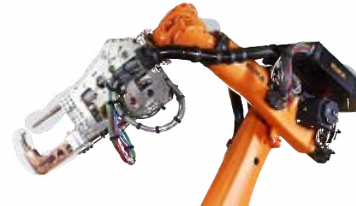
KUKA ready2_spot
